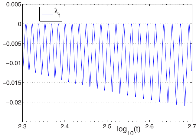
FIG. 4. (Color online) The finite-time flow Lyapunov exponent associated with an arbitrarily chosen trajectory in \mathcal{C} . Here a=0.03 . The local minima converge to the limiting value -a=-0.03 . Observe that the finite-time flow Lyapunov exponent function appears to converge to a periodic sawtooth function of \log(t) .
