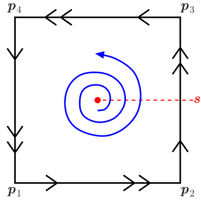
FIG. 3. (Color online) The flow on the square S = [0, \pi] \times [0, \pi] generated by (6).
