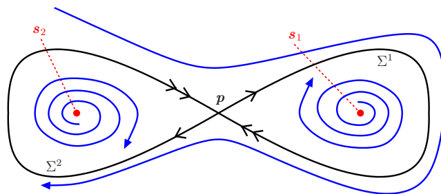
FIG. 1. (Color online) The figure-8 attractor. The point p is a saddle with more contraction than expansion, s_1 and s_2 are repelling foci, and the curves \Sigma^1 and \Sigma^2 are invariant loops. No trajectory that converges to the figure-8 has Lyapunov exponents except for the trajectories that start on the figure-8.
