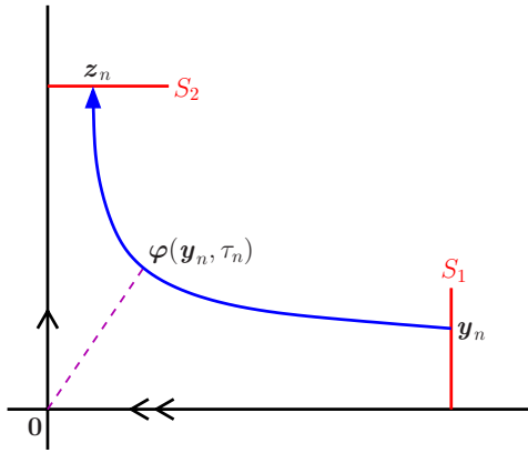
FIG. 2. (Color online) The flow from y_n to z_n .
